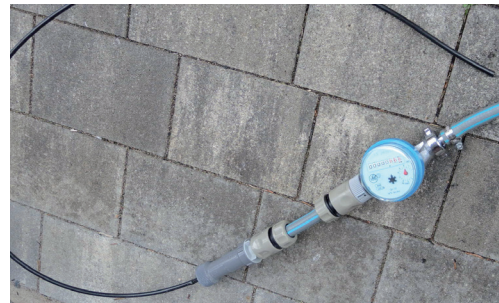
Figure 02: Flowmeter with garden hose and adapter for reducing to a thinner hose
