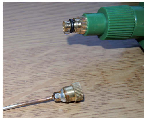
Figure 20: The nozzle of the spray bottle has been modified.
