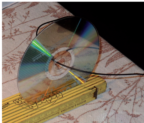
Figure 18: Water flows through a shrink-fit hose which passes through the hole in a DVD.
