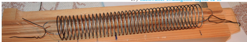
Figure 59: A helical spring is mounted in an adjustable holder which allows variation of the length. The tensile force is thus adjustable.
