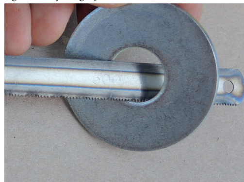
Figure 51: The hack-saw blade is pulled through a ferrite ring magnet.
