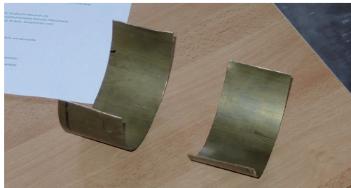
Figure 58: A brass pipe has been sawn into two sections. After the sawing process, the pipe has expanded diametrically. Evidently, mechanical stress was still present in the pipe, as a result of the drawing process during manufacture. strom-sehen-011.htm#kapitel-11
